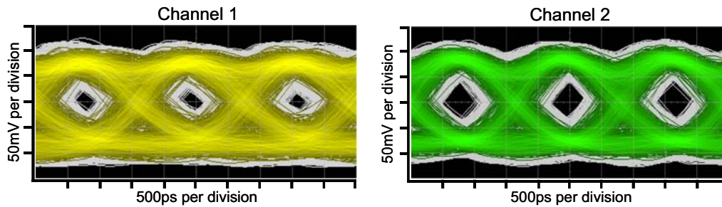
Figure 7: Eye patterns at 600Mbps
